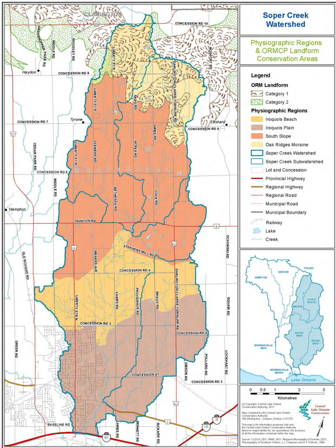
Figure 10: Soper Creek subwatershed physiographic regions and ORMCP Landform Conservation Categories (sources: Chapman and Putnam, 1984; MMAH, 2002).
