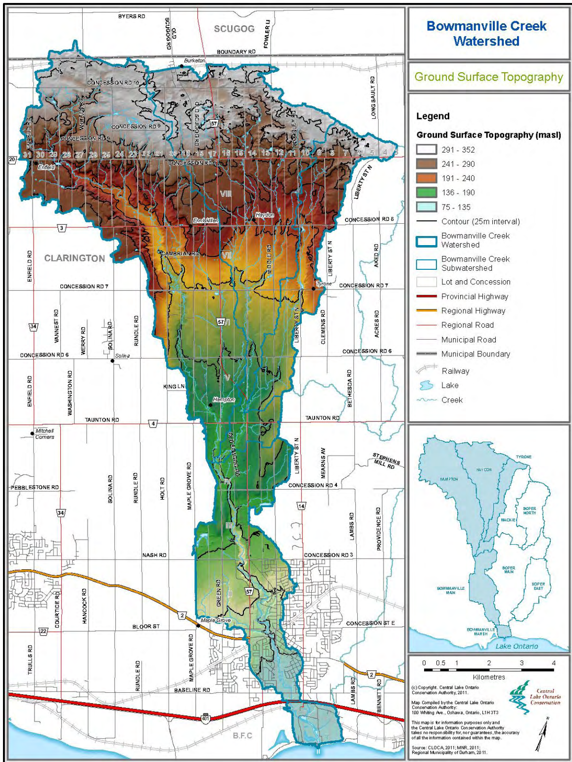
Figure 8: Bowmanville Creek subwatershed ground surface elevation
