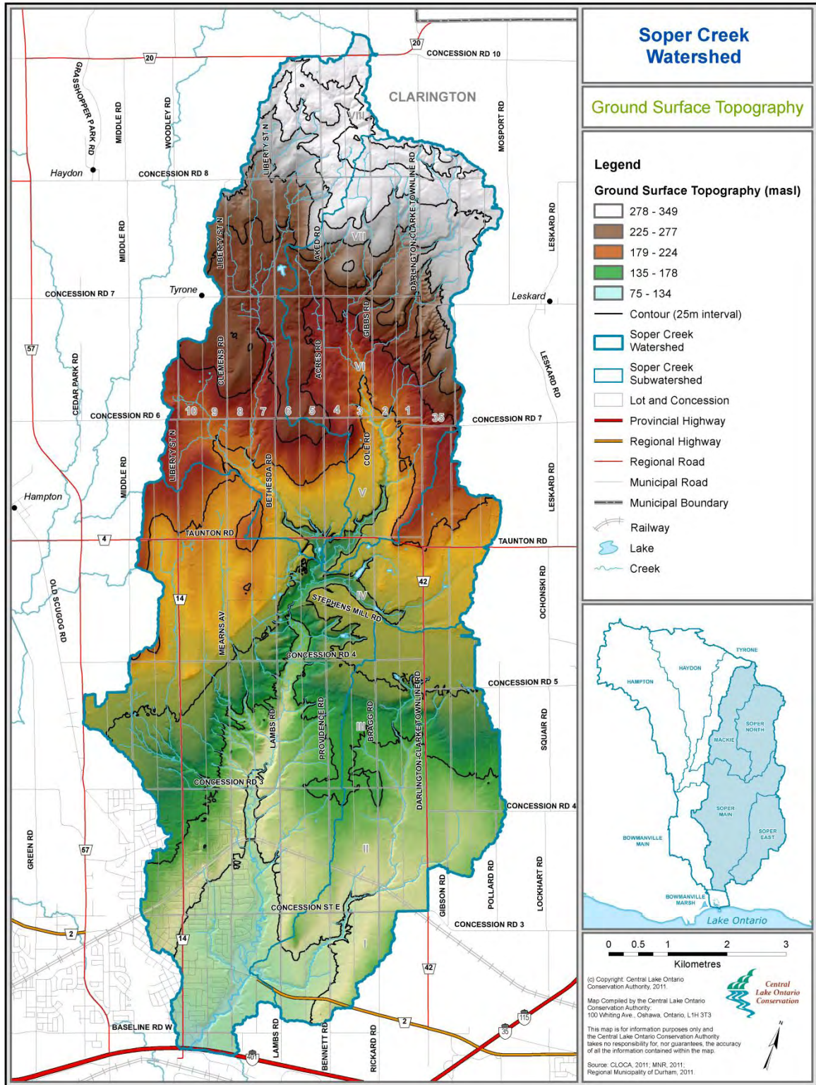
Figure 11: Soper Creek subwatershed ground surface elevation.
