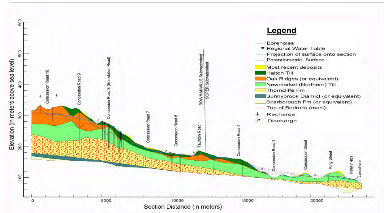
Figure 3: Bowmanville/Soper Creek watershed geological profile
