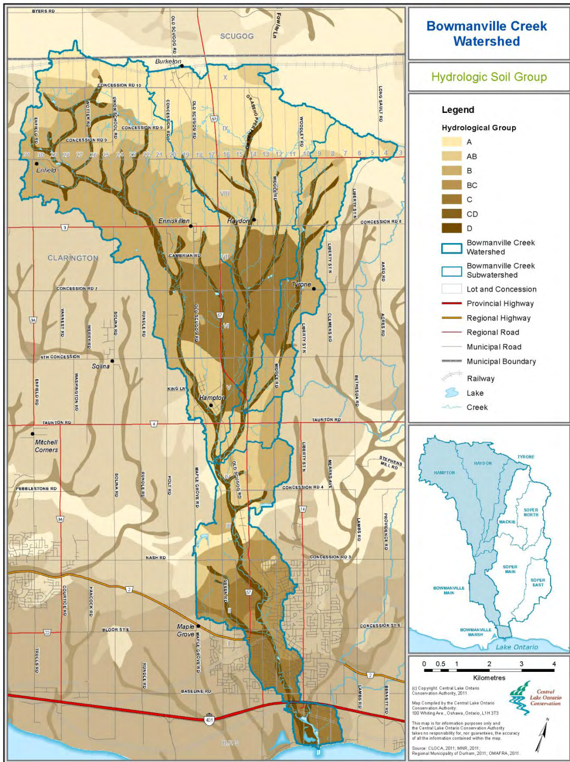
Figure 9: Bowmanville Creek subwatershed hydrologic soil groups (source: Ontario Ministry of Agriculture, Food and Rural Affairs, 1989).
