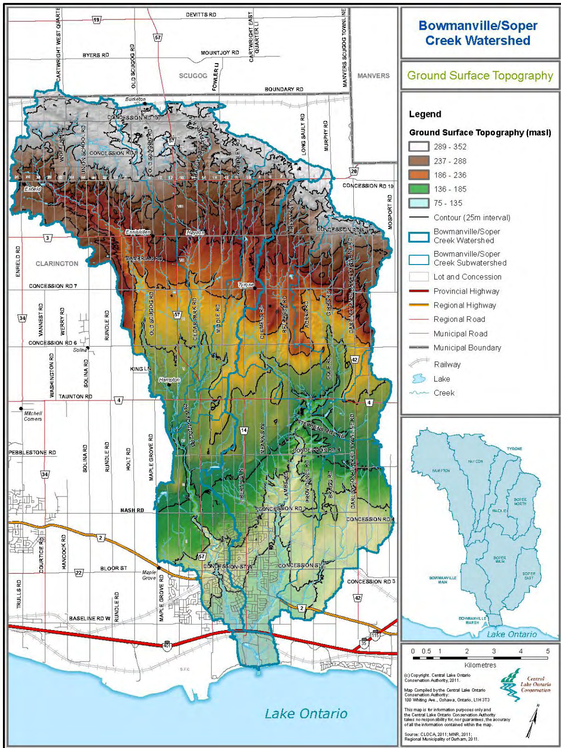
Figure 5: Bowmanville/Soper Creek watershed Ground surface elevation.
