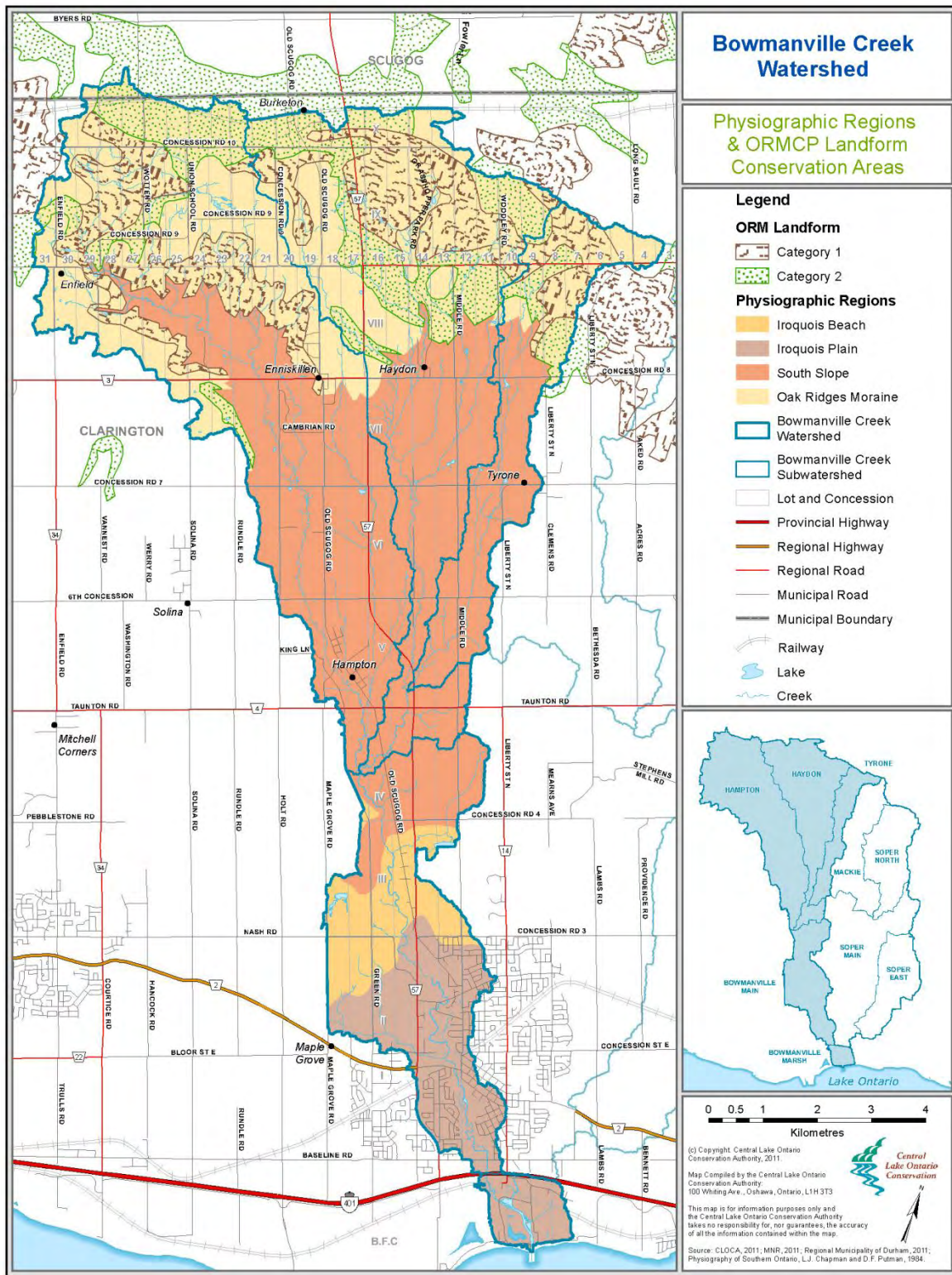
Figure 7: Bowmanville Creek subwatershed physiographic regions and ORMCP Landform Conservation Categories (sources: Chapman and Putnam, 1984; MMAH, 2002)
