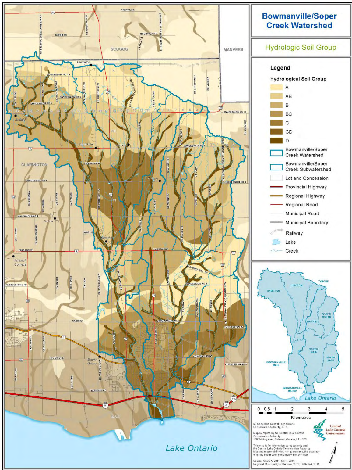
Figure 6: Hydrologic soil groups (source: Ontario Ministry of Agriculture, Food and Rural Affairs, 1989)
