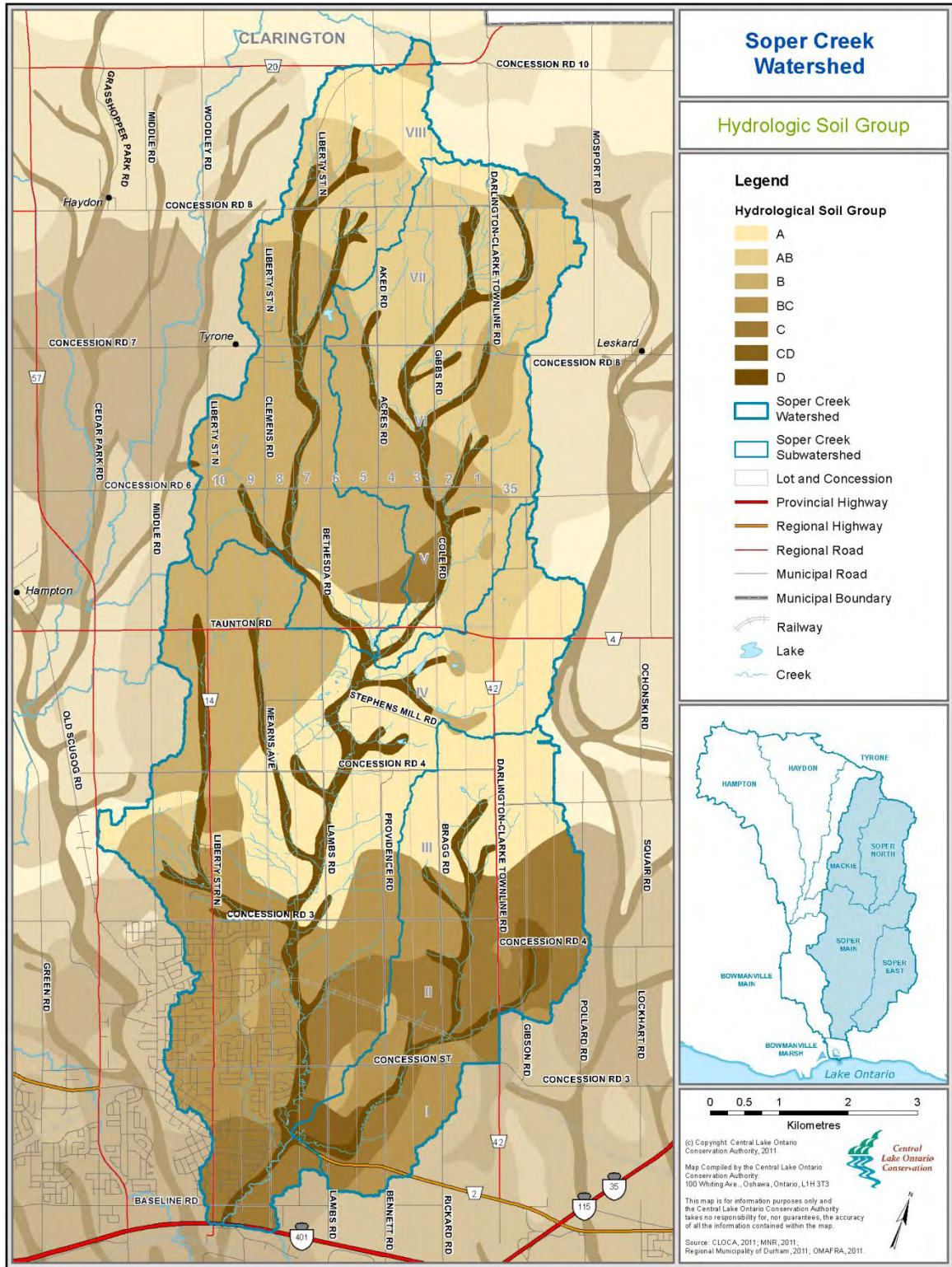
Figure 12: Soper Creek subwatershed hydrologic soil groups (source: Ontario Ministry of Agriculture, Food and Rural Affairs, 1989).
