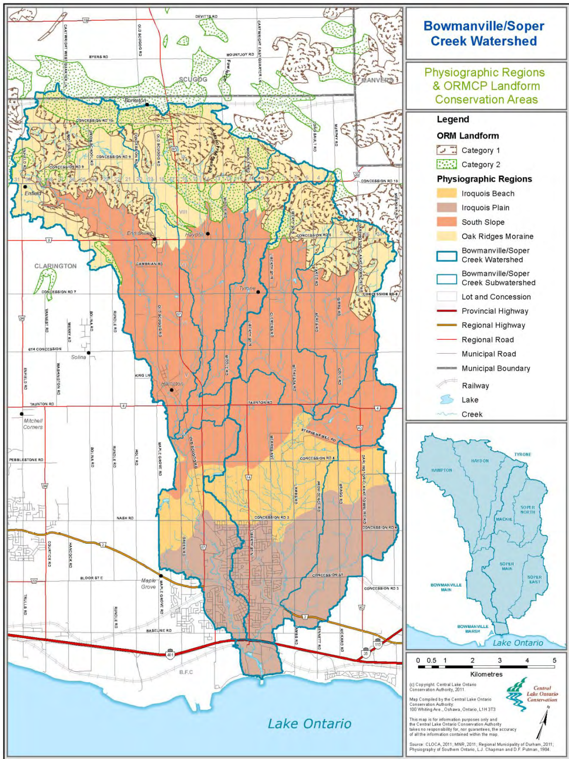
Figure 4: Physiographic regions and ORMCP Landform Conservation Categories (sources: Chapman and Putnam, 1984; MMAH, 2002).
