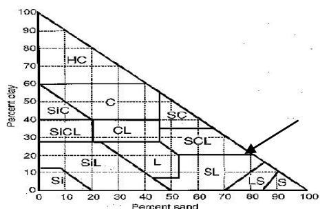
Figure 39 Soil texture classes triangle. Percentages of clay and sand in the main textural classes of soil; the remainder of each class is silt. Abbreviations for the texture classes are: HC, heavy clay; C, clay; SiC, silty clay; SiCL, silty clay loam; CL, clay loam; SC, sandy clay; SiL, Silt Loam; L, loam; SCL, sandy clay loam; SL, sandy loam; Si, silt; LS, loamy sand; S, sand.
